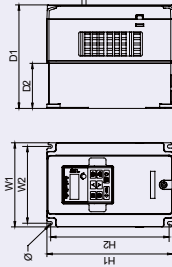
Wall mounting of 3PH 380V 4~37kW and 3PH 220V 1.5~7.5kW inverters
