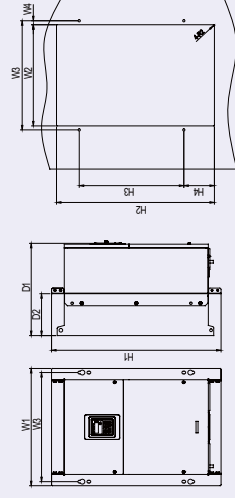
Flange mounting of 3PH 380V 90~110kW inverters
