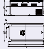
Wall mounting of 3PH 380V 4~7.5kW inverters
